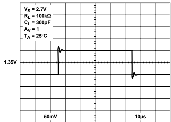
Figure 16. Small Signal Transient Response
