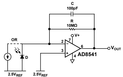
Figure 40. High Input Impedance Application—Photodiode Amplifier
