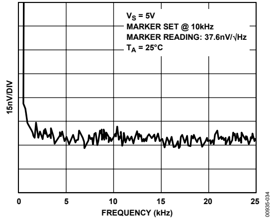
Figure 35. Voltage Noise
